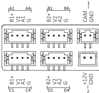
Figure 3-1 Terminals of Indoor Station
